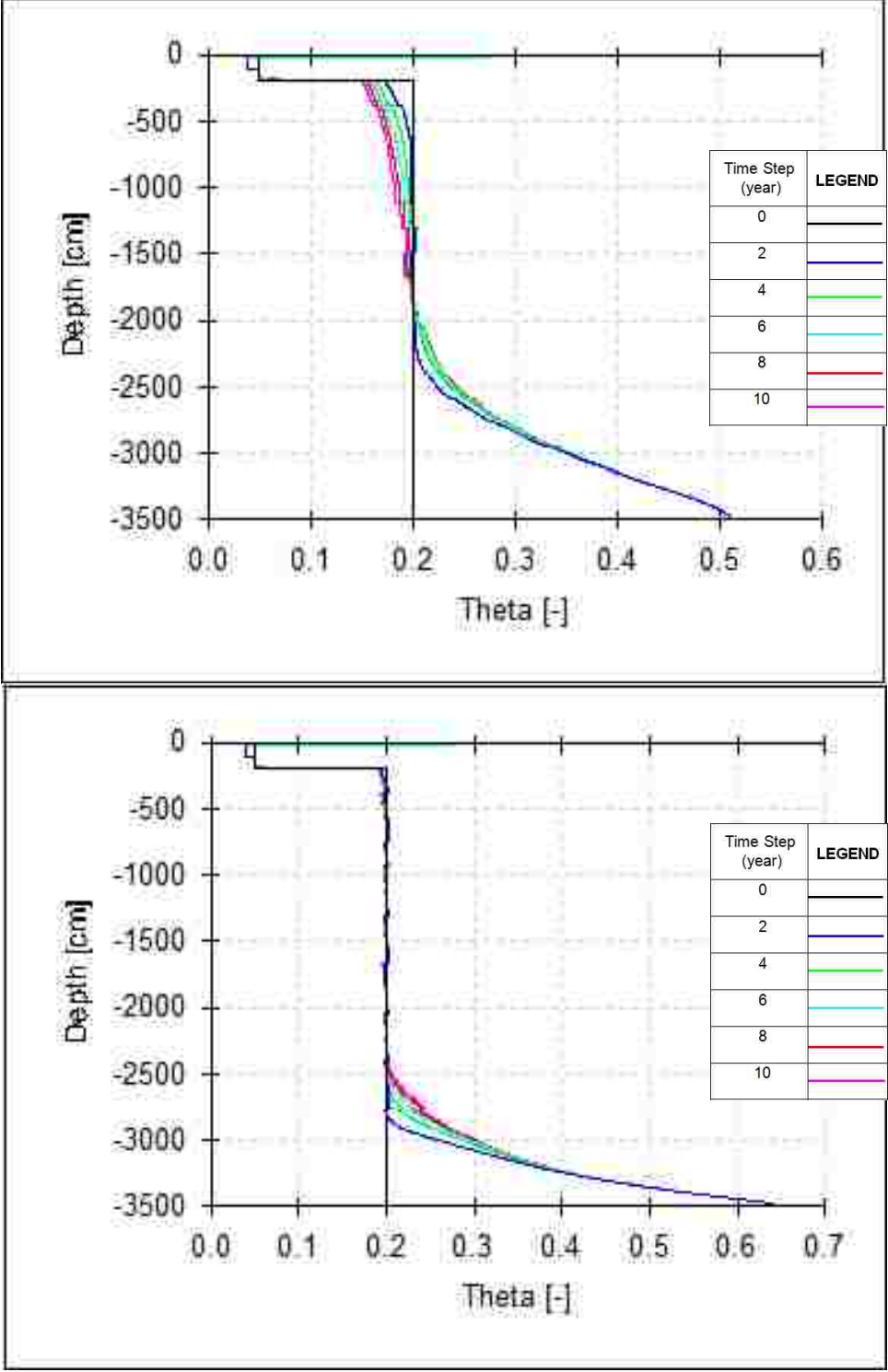
Figure 30: Water Table Present Water Content vs. Depth Results for Fly Ash(top) and Bottom Ash (bottom) Only Profiles
