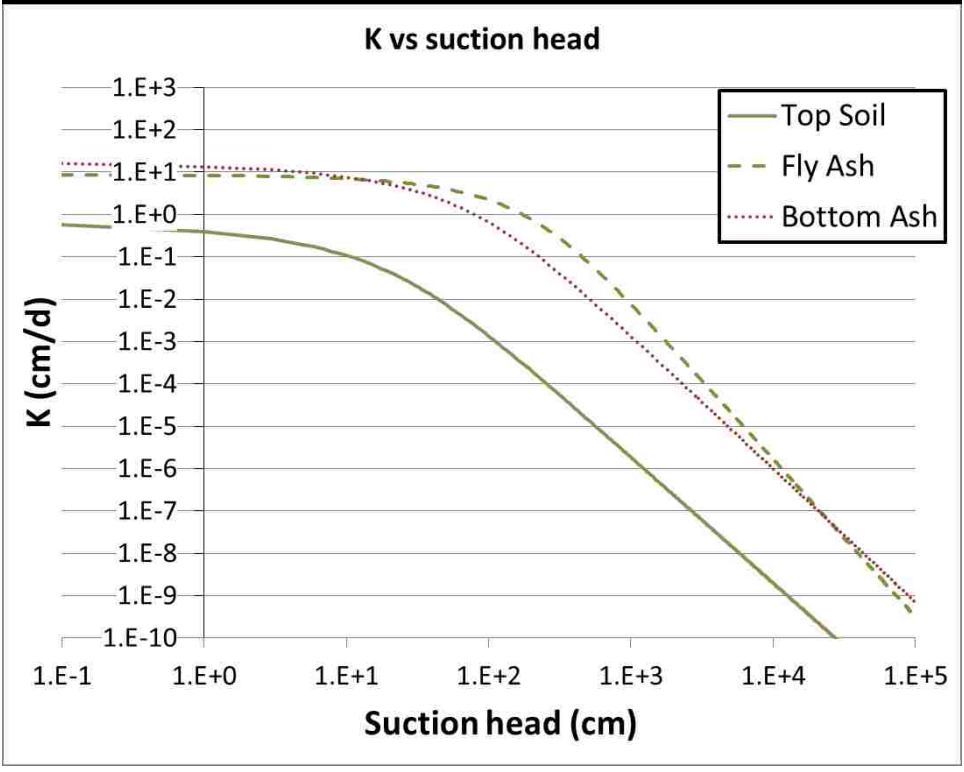
Figure 38: K vs. Suction Head for Top Soil, Fly Ash, and Bottom Ash at Interface between Top Soil and CCBs for Focused Recharge Simulations
