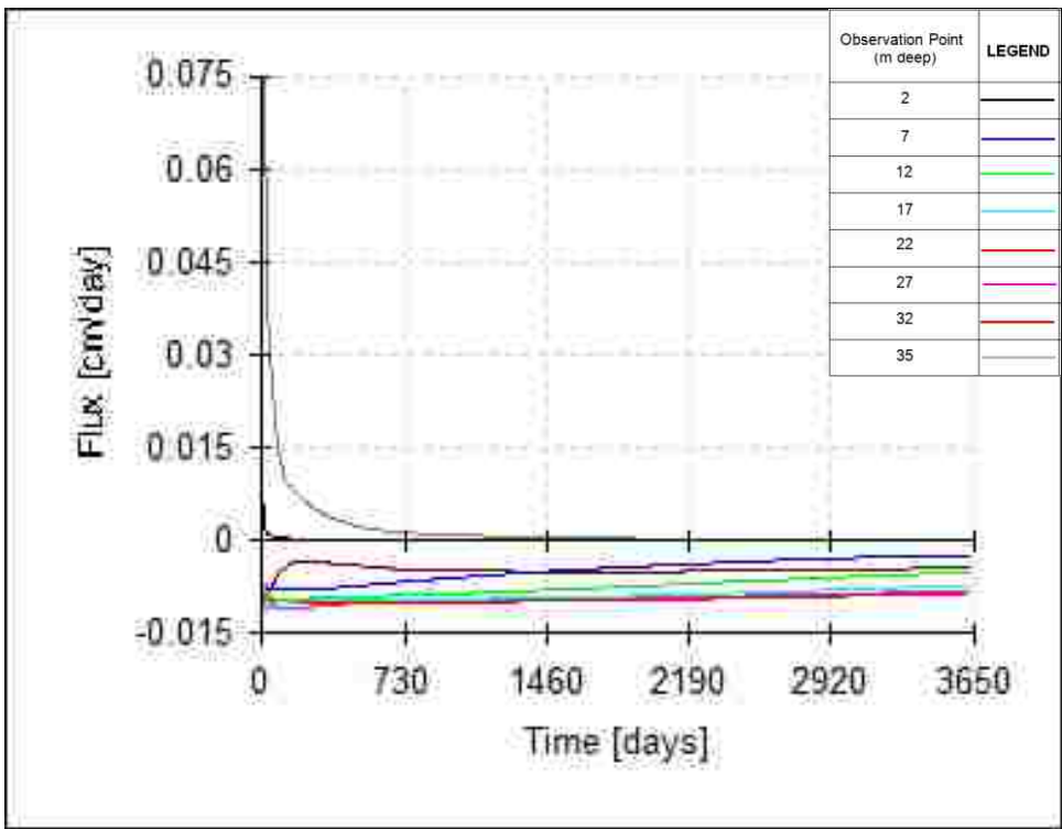
Figure 18: Baseline Results: Flux for Fly Ash Only Profile (top) and Bottom Ash Only Profile (bottom)
