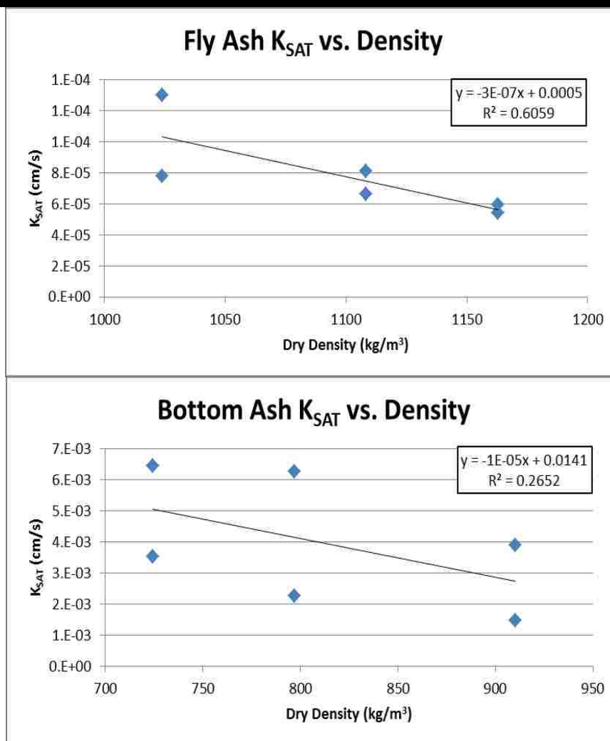
Figure 4: Saturated Hydraulic Conductivity vs. Dry Density Results
